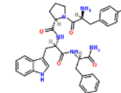
ENDORPHINE-1
