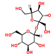
SUCROSE
