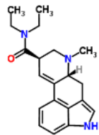
LSD
