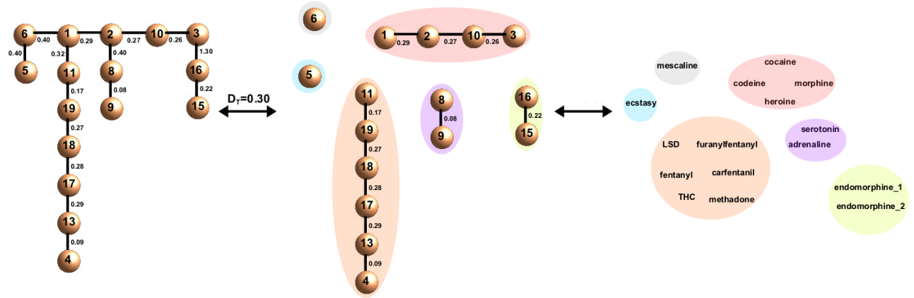
Figure 3: Minimum Spanning Tree Based on Euclidean Distances (nicotine, caffeine and sugar not included).
