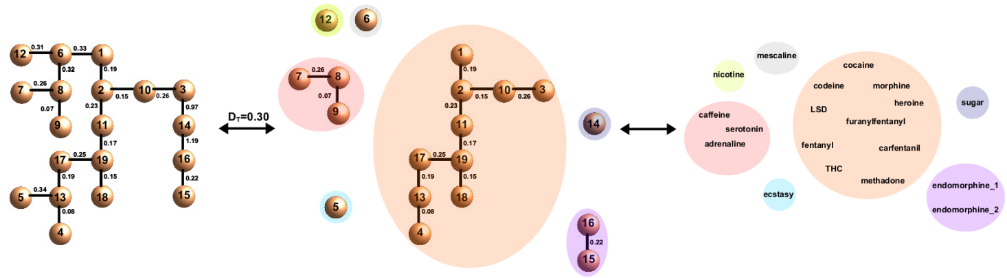
Figure 2: Minimum Spanning Tree Based on Euclidean Distances (full set of nineteen compounds).
