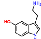
SEROTONINE
