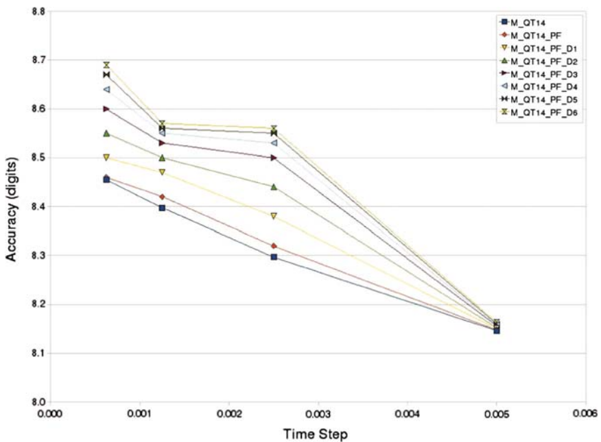
Fig. 3 The accuracy (digits) of the new methods compared to the classical one for the Schrödinger equation ( E = 341 )
