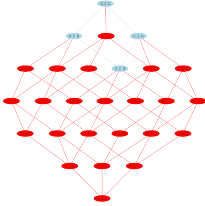
Fig. 2: A solutions tree example: blue nodes satisfy the k-anonymity requirements, while red nodes do not
